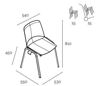
4-legs conference with joining hooks
